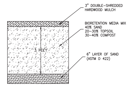
BIORETENTION CROSS SECTION
