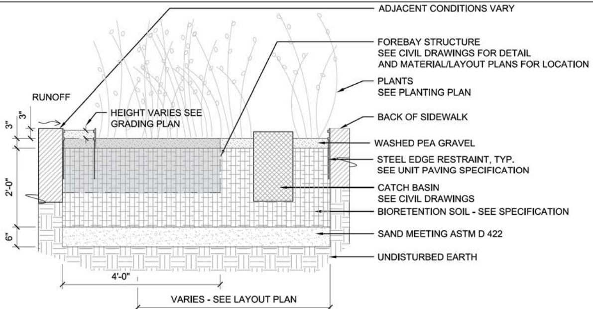
6 BIORETENTION PLANTER - TYPE B SCALE: 3/4" = 1'-0"
