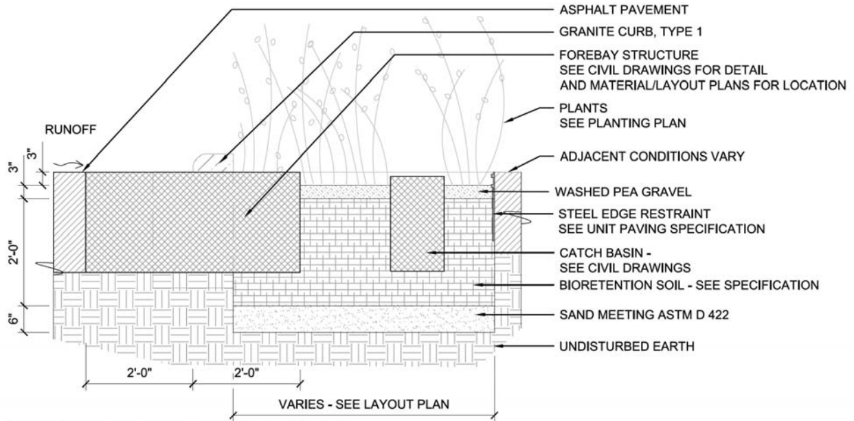
8 BIORETENTION PLANTER - TYPE A SCALE: 3/4" = 1'-0"
